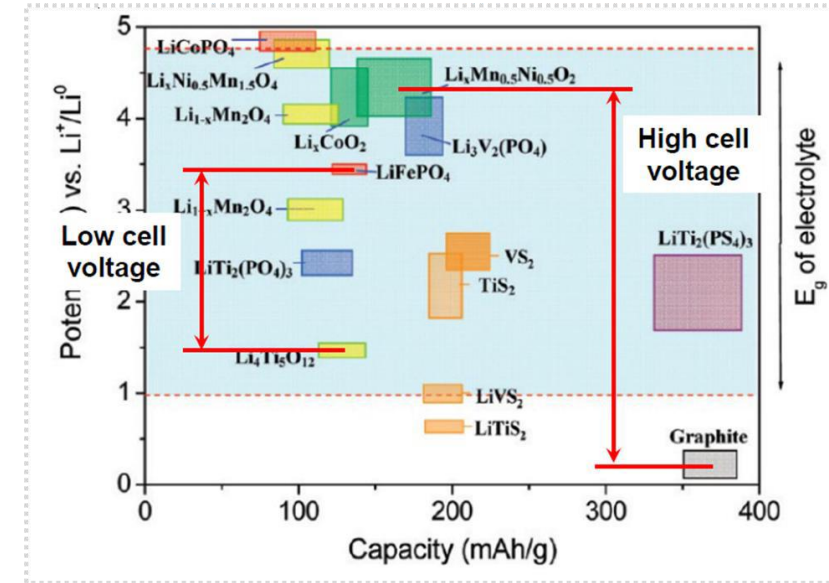
Li-ion technology choices
